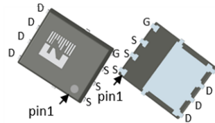
DFN5*6
